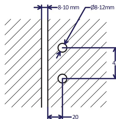
GLASS CUTOUT
