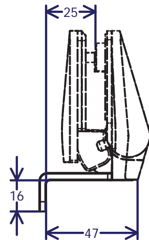
DIMENSIONS WITH HINGE
