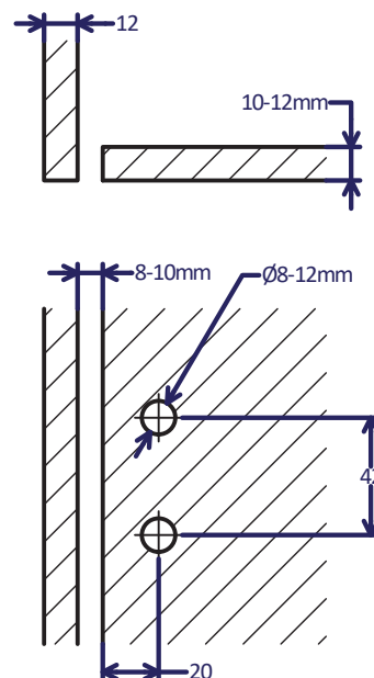
GLASS CUTOUT
