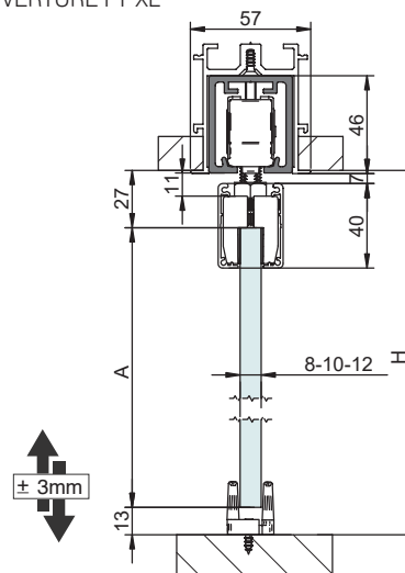
STAR XL + FUNDA I SUPPORT I COU- VERTURE FT XL
