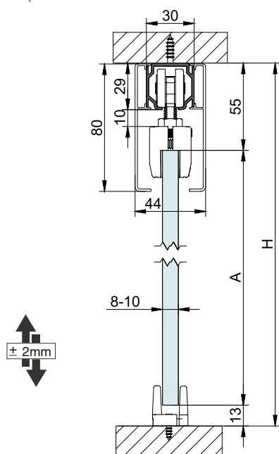
STANDARD A= H-68
