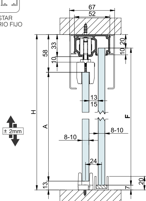
EXCELLENCE VIDRIO FIJO | FIXED GLASS | VERRE FIXE
