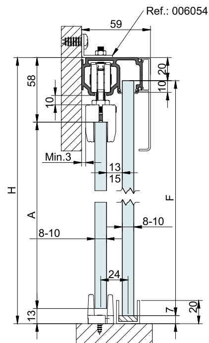
EXCELLENCE VIDRIO FIJO | FIXED GLASS | VERRE FIXE
