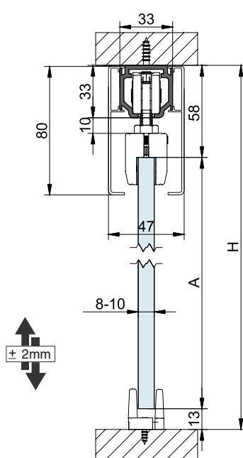
EXCELLENCE A= H-71
